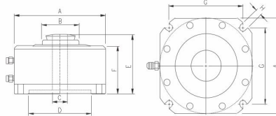
JAS-15/JAS-25/JAS-5C (Collet Style)
