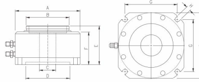
JAS-40/JHS-40/JHS-70 (Jaw Style)
